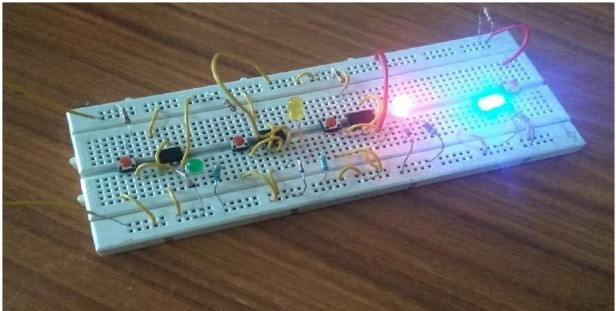
Fastest Finger First
