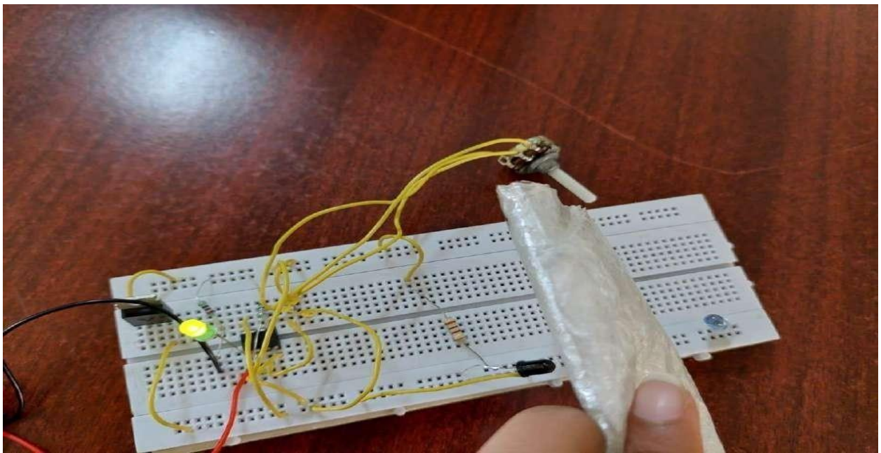
Home Security using IR sensor
