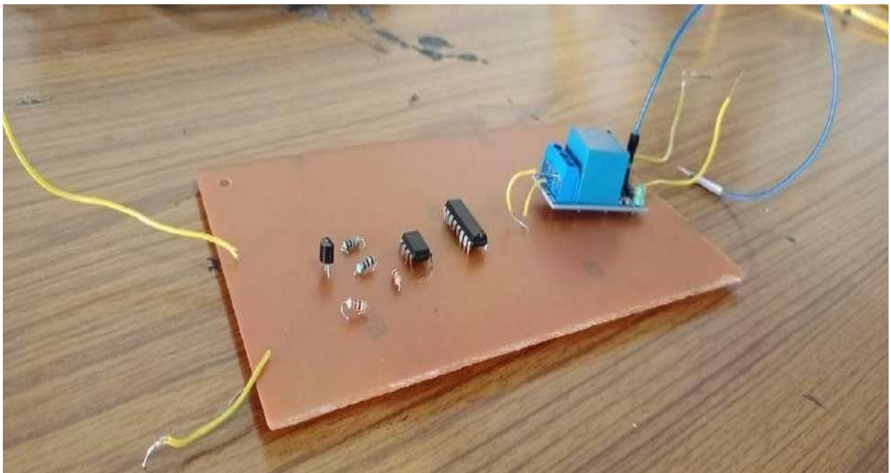
Automatic Washroom Light Switch
